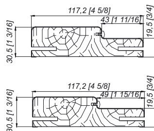
Jamb Type 80/5/116 (quartered 49 and 43)
